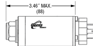
Fixed Plug to DIN 43650 Mating Connector Supplied
