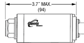
Six Pin Fixed Plug (10-6)
