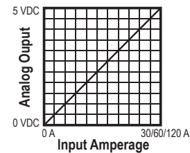
Figure 9: CTCGV05NN Linear Output
