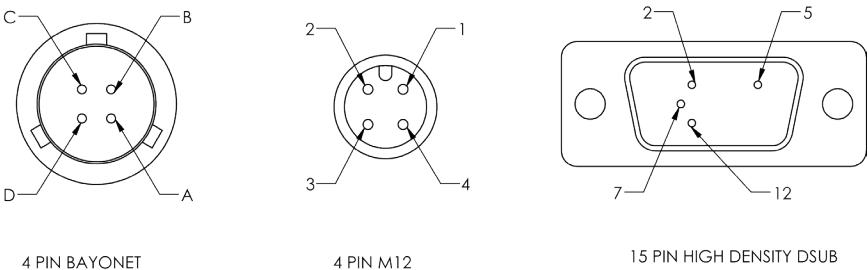
Diagram 2: Transducer Pin out
